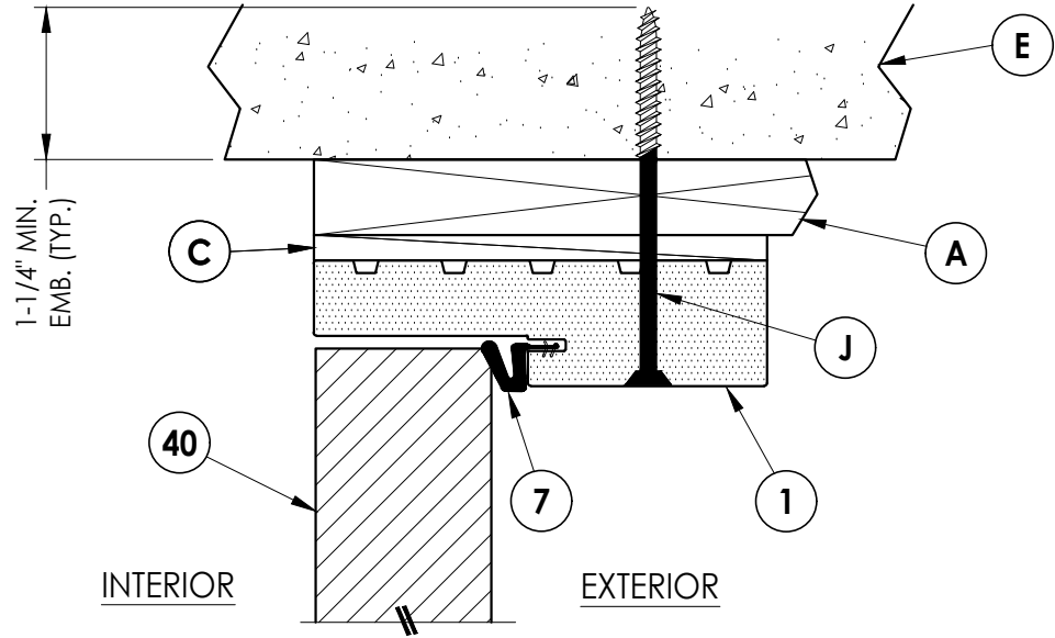
3 6 VERTICAL CROSS SECTION Shown w/ 1X sub-buck Inswing shown (Outswing similar)
