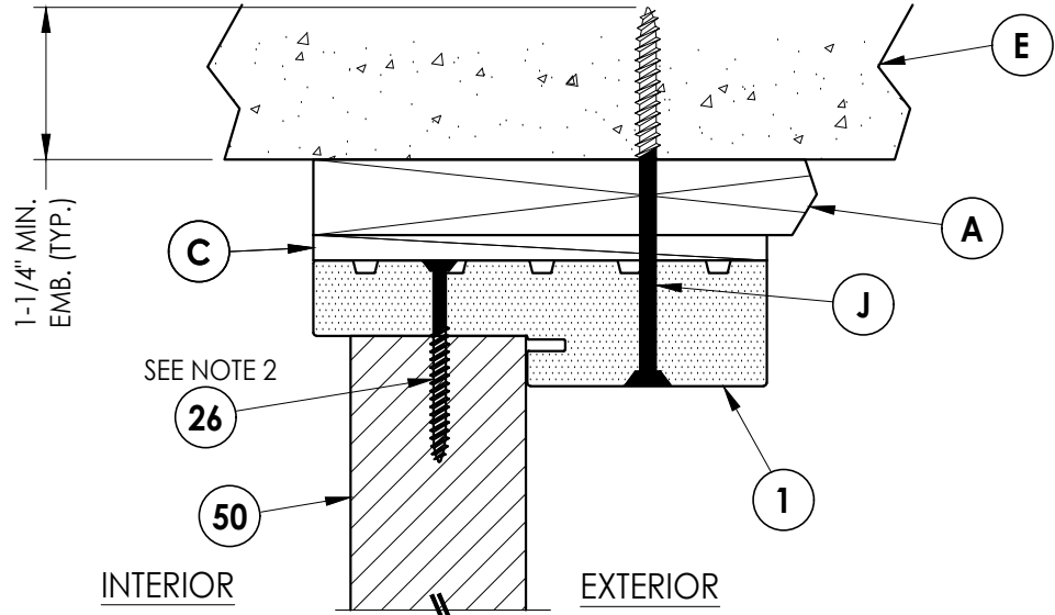
4 6 VERTICAL CROSS SECTION Shown w/ 1X sub-buck Inswing shown (Outswing similar)
