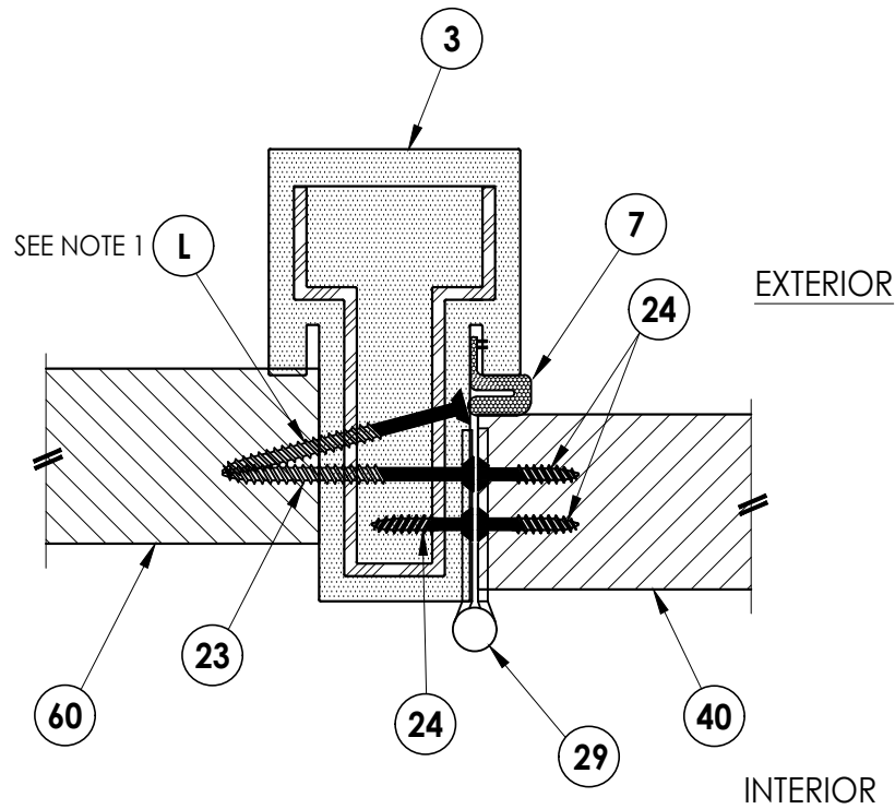
5 5 HORIZONTAL CROSS SECTION Inswing shown (Outswing similar)
