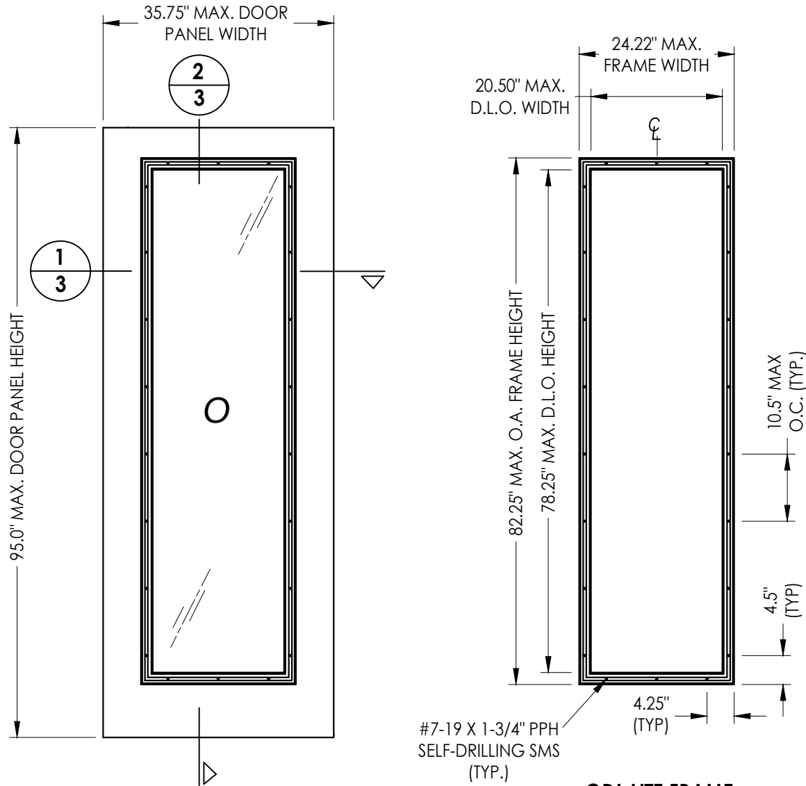
50 SIDELITE PANEL Mastergrain
