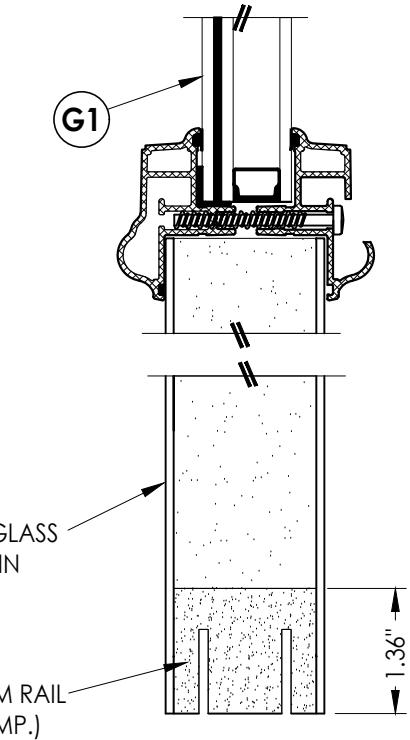
2 3 VERTICAL CROSS SECTION
