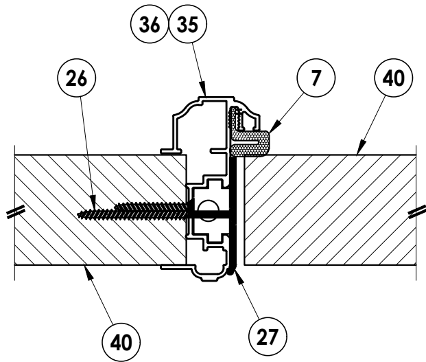
6 5 HORIZONTAL CROSS SECTION Inswing shown (Outswing similar)
